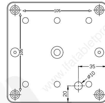
Back view unit: mm
