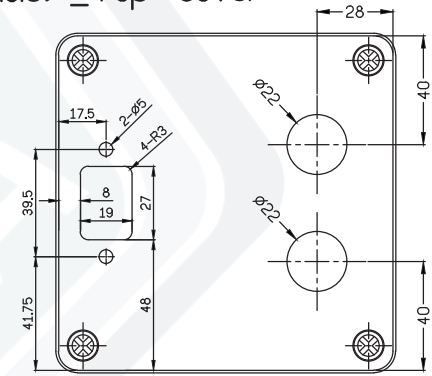
Upper view unit: mm
